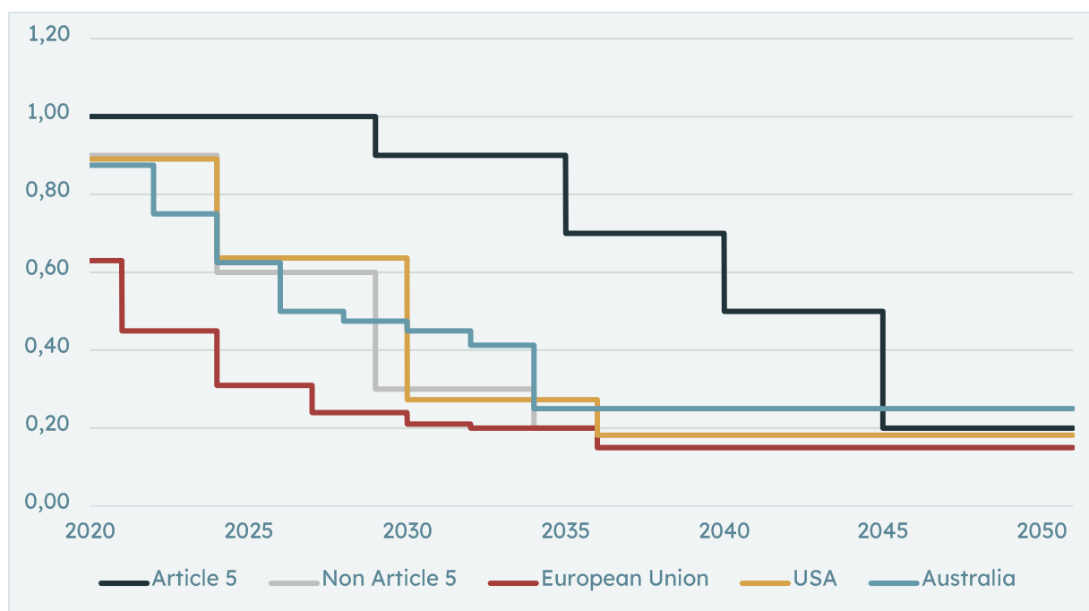
Figure 23 Global Phase Down for F-Gases
