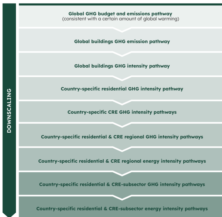
Figure 3 Schematic overview of the CRREM downscaling methodology
