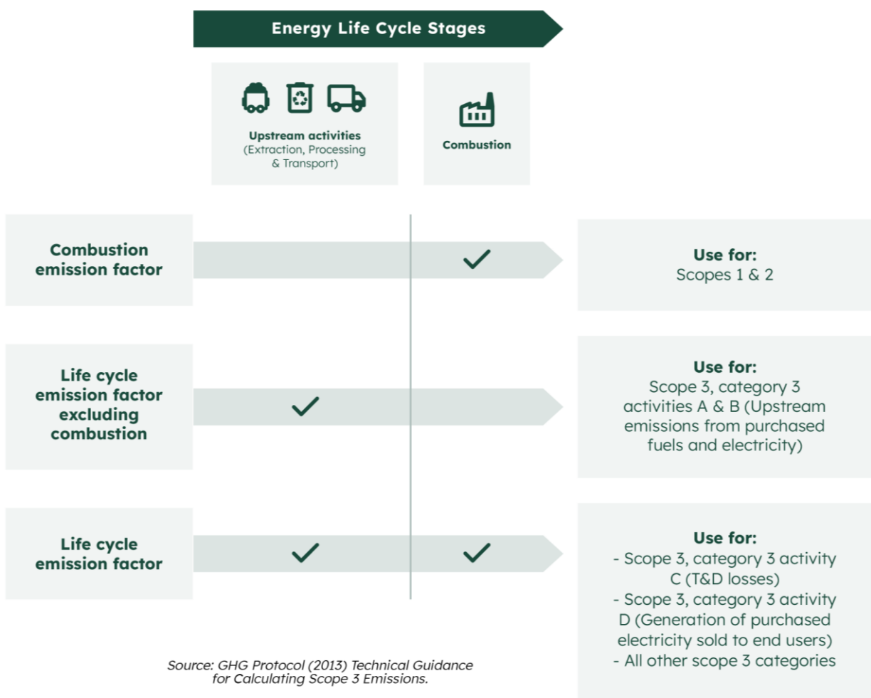
Figure 7 Treatment of T&D-losses according to GHG protocol
