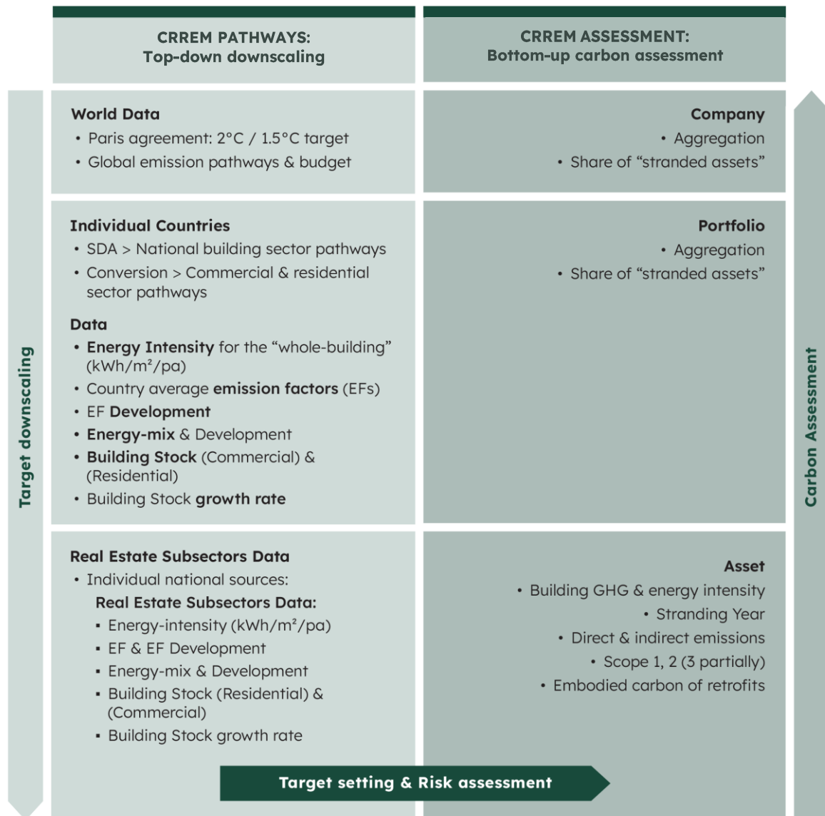
Figure 2 Overview of downscaling approach for target setting and carbon risk
