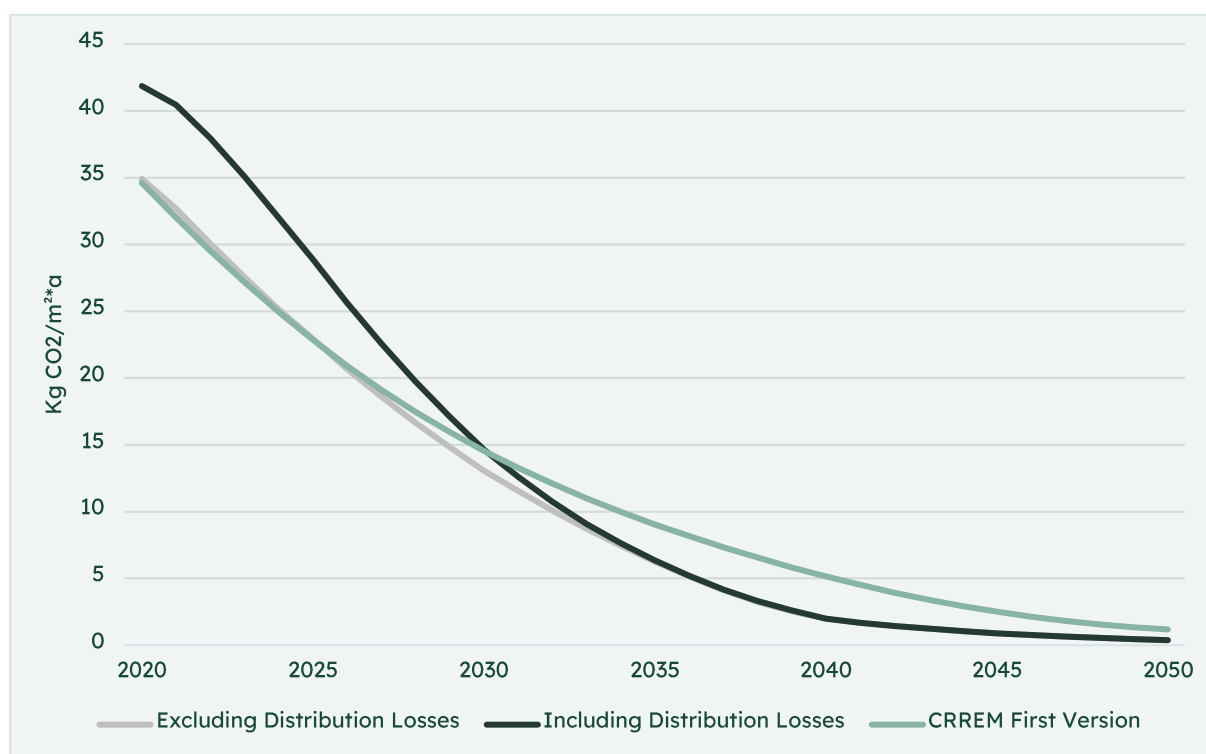
Figure 8 Global building sector CO 2 -only intensity pathways (excluding vs. including T&D-losses) 21
