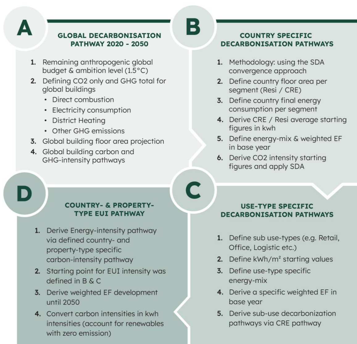
Figure 5 Steps of the CRREM downscaling-methodology
