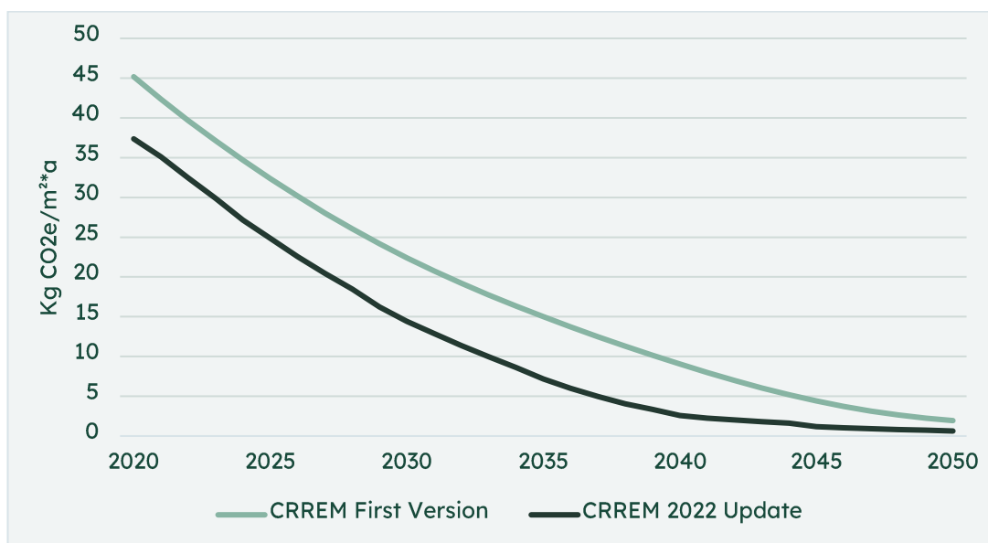
Figure 17 Global building sector CO 2e intensity pathways
