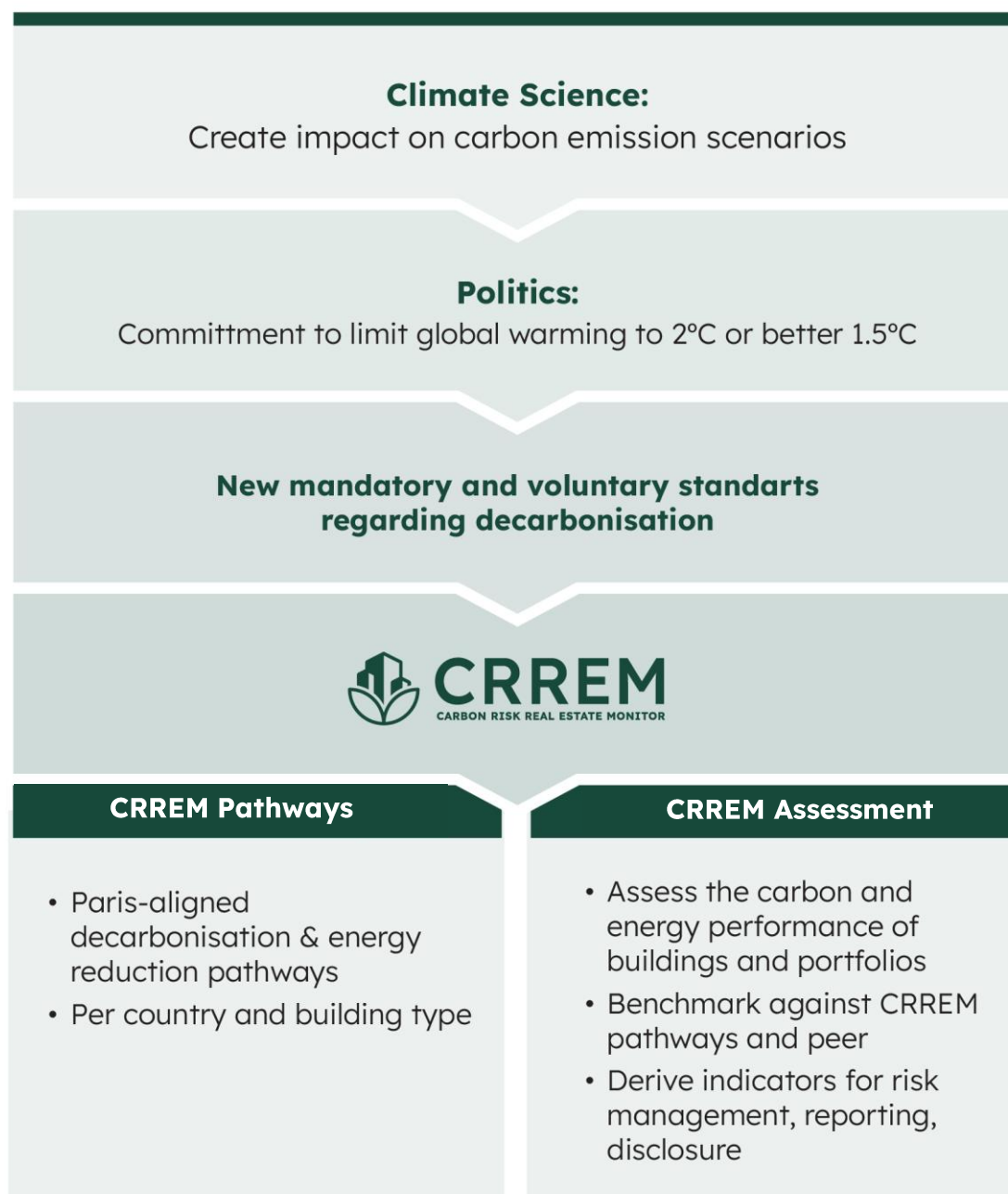
Figure 1 From climate science to decarbonization pathways and carbon risk indicators
